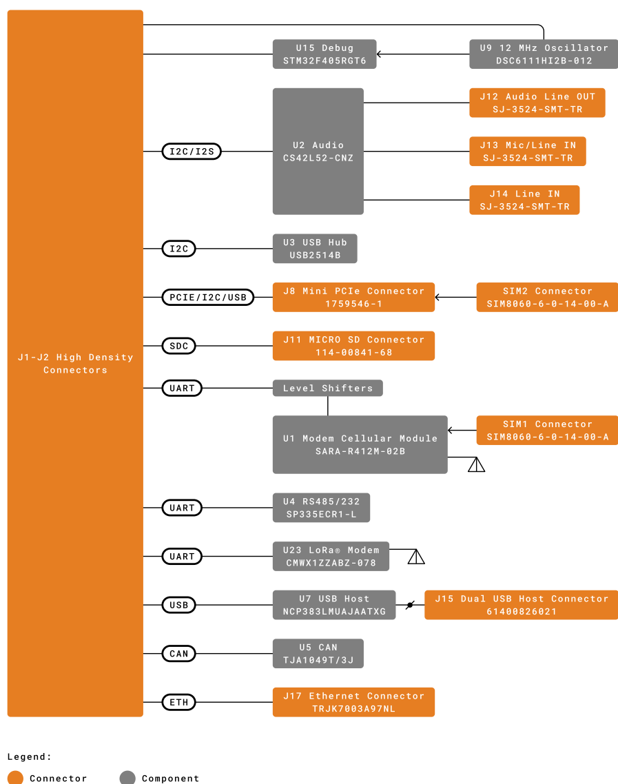
Block Diagram
